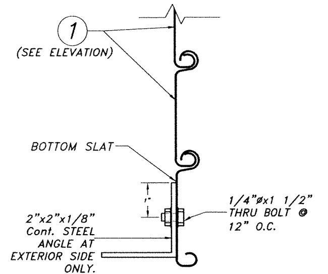
SECTION X1
