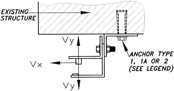
LOAD DIAGRAM: "Z" GUIDE
