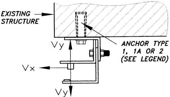
LOAD DIAGRAM: "E" GUIDE
